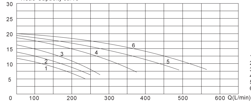
H(m) Head-Capacity curve
